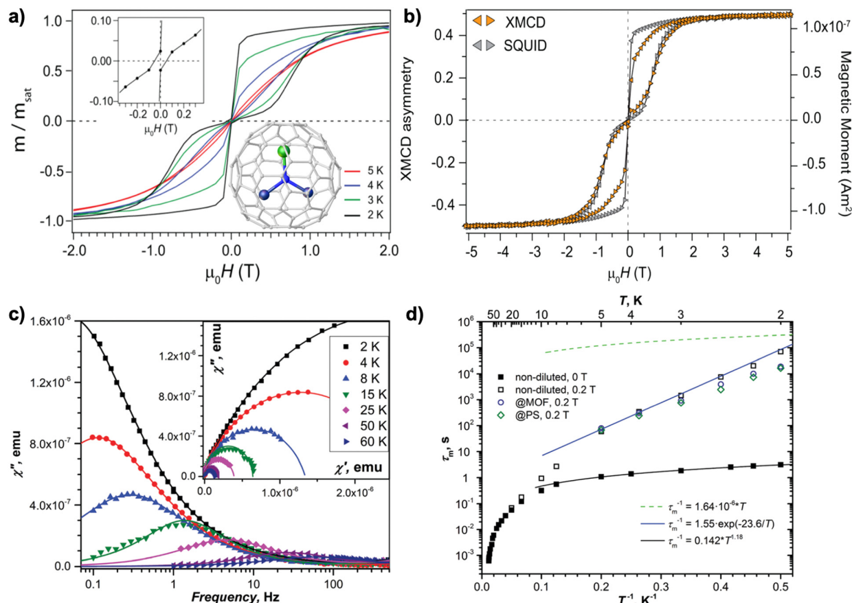
Fig. 2 (a) Magnetic hysteresis loops for \text{DySc}_2\text{N}@\text{C}_{80} (the molecular structure is shown in the inset) recorded using SQUID magnetometry at 2–5 K with a field sweep rate of 1.3 \text{ mT s}^{-1} . (b) Comparison of the magnetic hysteresis loops for \text{DySc}_2\text{N}@\text{C}_{80} recorded by SQUID and XMCD magnetometry at 2 K. Reproduced with permission from ref. 15 (Copyright 2012, American Chemical Society). (c) Out-of-phase magnetic susceptibility \chi'' of \text{DySc}_2\text{N}@\text{C}_{80} measured in zero field in the 2–60 K range. The inset shows Cole–Cole plots. The solid lines are fits by the generalized Debye model. (d) Magnetization relaxation times of \text{DySc}_2\text{N}@\text{C}_{80} at temperatures of 2–87 K. Zero-field values are shown as full dots and in-field (0.2 T) values are denoted as open dots. Relaxation times for non-diluted \text{DySc}_2\text{N}@\text{C}_{80} are shown in black, and the values for diluted samples are shown in blue (diluted with MOFs) and green (diluted with polystyrene, PS). Reproduced from ref. 64.
