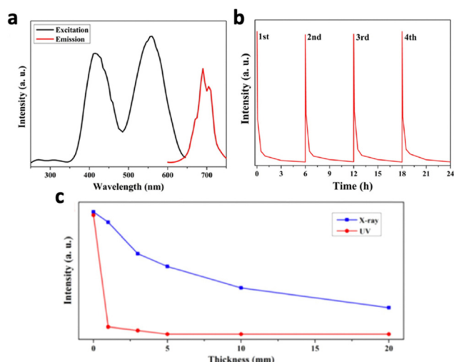
Fig. 18 (a) Excitation spectrum (black) and emission spectrum (red) of \text{ZnGa}_2\text{O}_4:\text{Cr}^{3+} . (b) 4 Cycles of persistent luminescence decay curves by \text{ZnGa}_2\text{O}_4:\text{Cr}^{3+} following cessation of X-ray irradiation (5 min, 45 kVp). (c) Luminescence intensity of \text{ZnGa}_2\text{O}_4:\text{Cr}^{3+} excited by X-ray (blue) and 365 nm UV (red) through pork tissues with different thicknesses (0, 1, 3, 5, 10, and 20 mm). Reproduced with permission from ref. 211. Copyright 2017, American Chemical Society.
