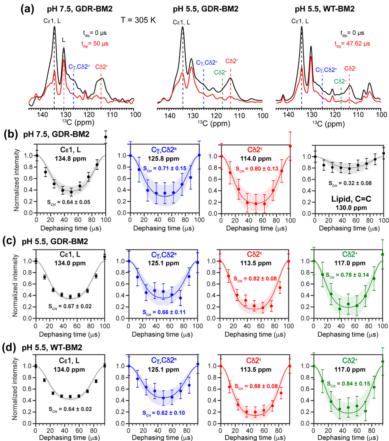
Fig. 6 2\text{D }^{13}\text{C}-^1\text{H} DIPSIFT data of membrane-bound GDR-BM2 and WT-BM2. The spectra were measured at 305 K under 10 kHz or 10.5 kHz MAS. (a) Aromatic region of the ^{13}\text{C} dimension of the 2D spectra of the three peptides at C-H dipolar evolution times of 0 \mu\text{s} and half of the rotor period (50 \mu\text{s} or 47.6 \mu\text{s} ). (b) C-H dipolar dephasing of GDR-BM2 at pH 7.5. (c) C-H dipolar dephasing of GDR-BM2 at pH 5.5. (d) C-H dipolar dephasing of WT-BM2 at pH 5.5. Error bars were propagated from the spectral signal-to-noise ratios. Best-fit simulations (solid lines) are shown along with uncertainties in the S_{\text{CH}} values (shaded areas) up to two standard deviations. The rigid-limit C-H dipolar coupling is assumed to be 23.9 kHz.
