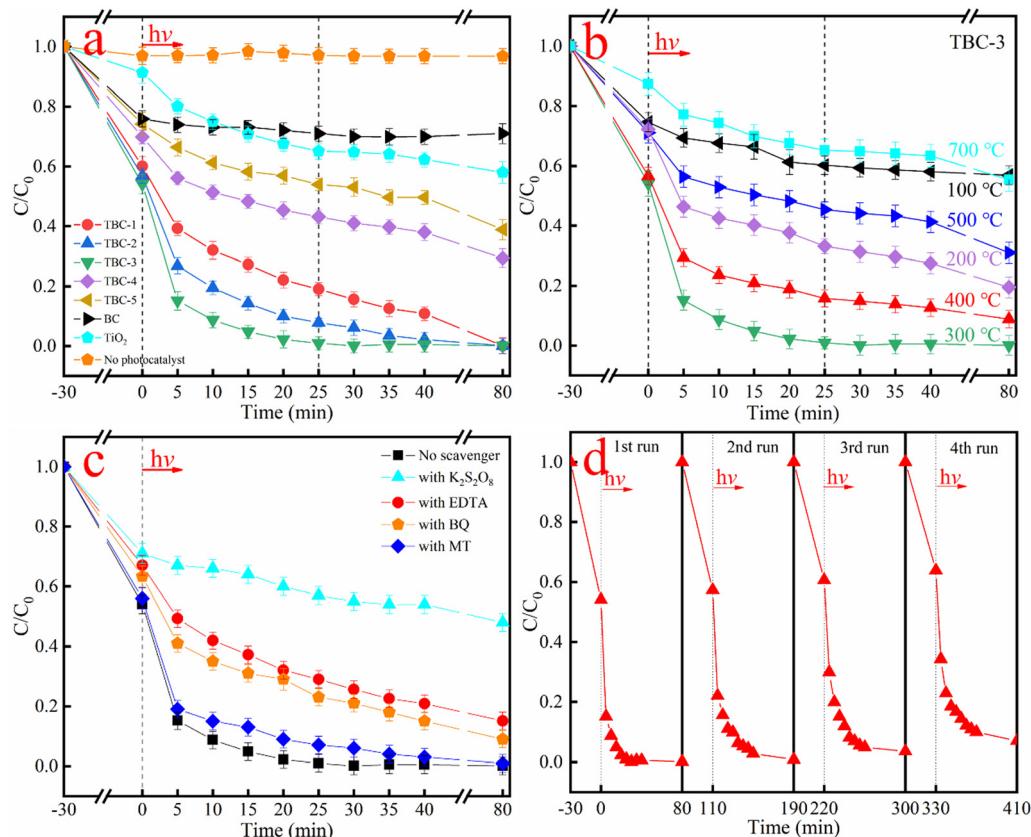
Fig. 9 Absorption-photocatalytic reduction of Cr(vi) with BC, TiO 2 and TBC samples (a), with TBC-3 calcined at different temperatures (b) and over TBC-3 composite in the presence of K 2 S 2 O 8 , EDTA, BQ and MT scavengers (c). Recycling experiments using TBC-3 composite for the absorption-photocatalytic reduction of Cr(vi) (d).
