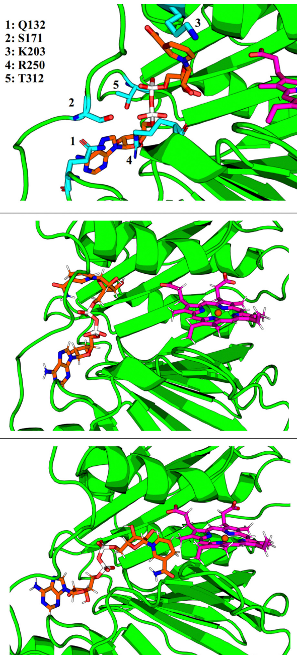
Fig. 8 Top: Close-up representation of the holo -HemS main pocket with NADH (computational reconstruction). NADH is shown in orange. The most important residues implicated in NADH-binding are shown in cyan. Middle: Representative structure of folded NADH docking to the heme-binding cavity. Bottom: Representative structure of unfolded NADH, where it can access heme.
