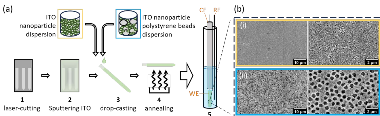
Figure 1. Overview of FE-EPR set-up, working electrode assembly process and structure. (a) Production and assembly of mesoporous and inverse-opal mesoporous ITO working electrodes: 1 laser-cutting Ti strips out of Ti foil; 2 sputtering a layer of ITO onto Ti strips; 3 drop-casting the dispersion on to the sputtered strips; 4 annealing the strips at 500 °C; 5 resulting working electrode (WE) assembled in the FE-EPR set-up in a 4 mm O.D. EPR tube, with the reference electrode (RE) position at 2.5 cm from the bottom of the tube, at half the length of the WE; all the electrodes are submerged in 300 µL of electrolyte solution. (b) SEM images of the ITO structures of (i) mesoITO and (ii) IO-mesoITO working electrodes.
