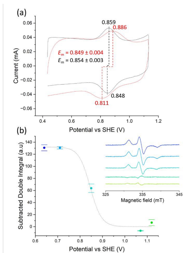
Figure 2. Benchmarking of the modified PFE-EPR set-up using amino-TEMPO. (a) Cyclic voltammograms in a standard electrochemical cell (black) and in the PFE-EPR cell (red) at 10 \text{ mVs}^{-1} . (b) Titration curve resulting from plotting the double integral of the EPR spectra (100 K) of different electrodes vs the specific potentials that they were poised at. The dotted line represents the fit to the Nernst equation with n = 1 and E_m = +0.853 \text{ V} vs SHE. The inset shows the averaged EPR spectra acquired at 100 K after subtraction of unreacted amino-TEMPO.
