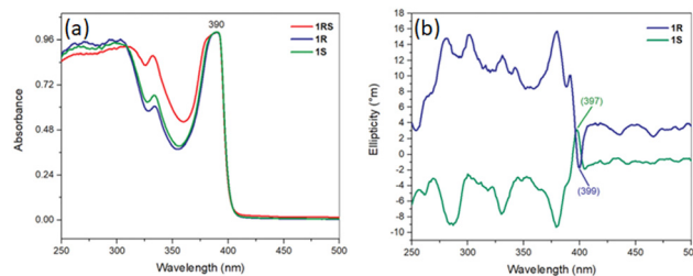
Fig. 14 (a) UV visible absorption and (b) CD spectra of (R/S\text{-Mpa})_2\text{PbBr}_4 . Reprinted with permission from ref. 35 Copyright©2020 Royal Society of Chemistry.
