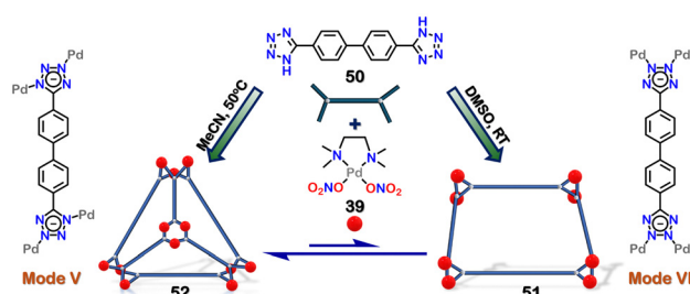
Fig. 18 Schematic representation for the formation of 51 molecular square ( 51 ) and 3D-tetrahedral cage ( 52 ) and the dynamic reaction between 51 and 52 , along with the representation of the dual binding modes adopted by 50 .
