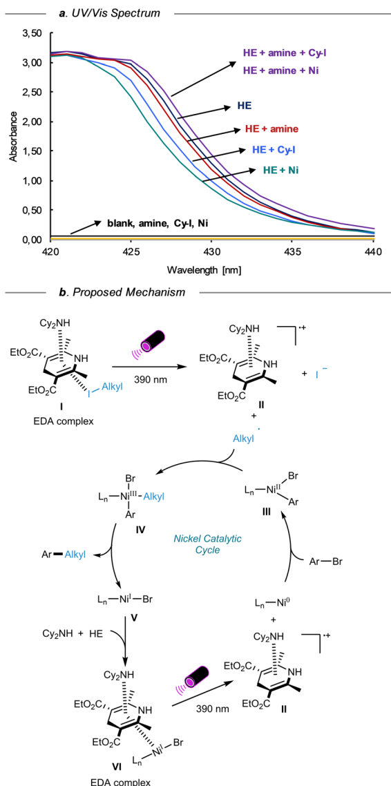
Scheme 3 UV-vis absorption study and proposed mechanism.
