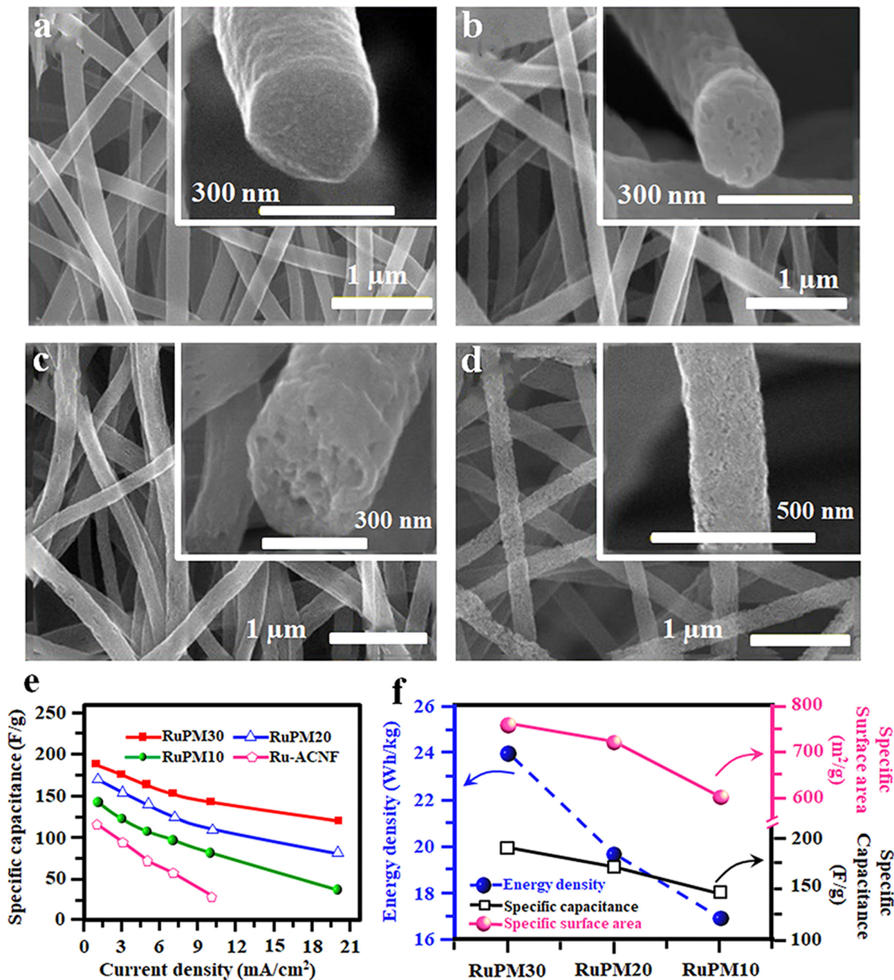
Fig. 9 (a)–(d) FE-SEM micrographs of the Ru-ACNF webs obtained using different concentrations of PMMA after activation. (e) Variation of specific capacitance at different current densities and (f) variation of surface area, specific capacitance and energy density of SC electrodes with PMMA concentration. Reproduced from ref. 100 with permission from Elsevier, copyright 2016.
