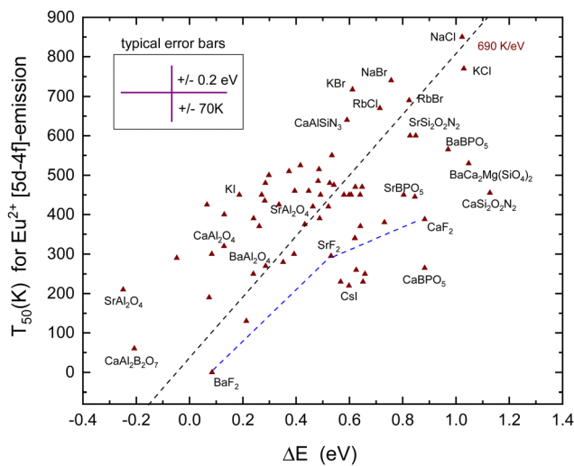
Fig. 7 T_{50} quenching data of the \text{Eu}^{2+} 5d–4f emission against the energy difference \Delta E between the relaxed 5d-state and the CB-bottom. Data points for \text{MF}_2 ( M = \text{Ba, Sr, Ca} ) compounds are connected by straight line segments. The typical error bars are shown.
