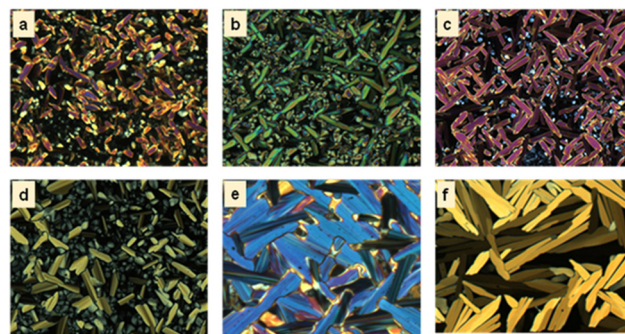
Fig. 3 POM microphotographs of the optical texture of Col phases formed by (a) P-5 at 280 ^\circ\text{C} , (b) P-6 at 230 ^\circ\text{C} , (c) P-7 at 225 ^\circ\text{C} , (d) P-8 at 190.7 ^\circ\text{C} , (e) P-10 at 150.9 ^\circ\text{C} and (f) P-11 at 214.9 ^\circ\text{C} .
