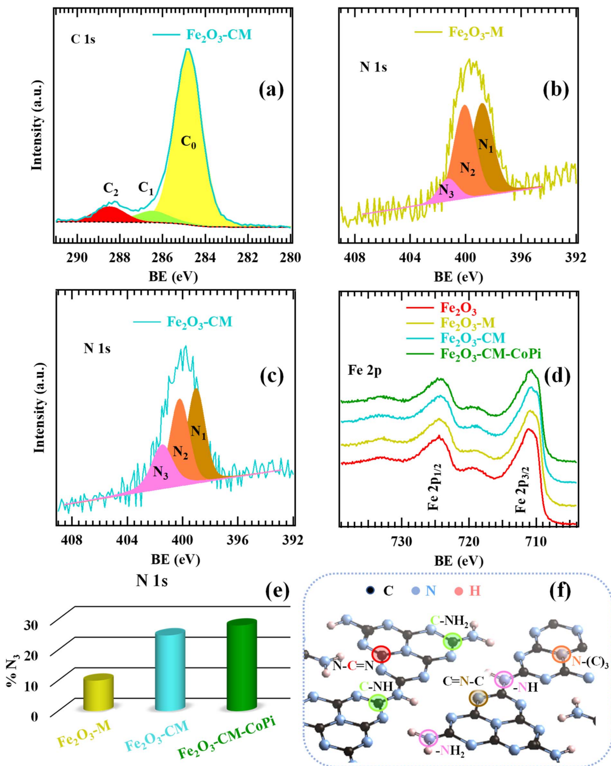
Fig. 2 XPS surface characterization: C 1s (a), N 1s (b and c) and Fe 2p (d) photoelectron peaks for \text{Fe}_2\text{O}_3 -M and \text{Fe}_2\text{O}_3 -CM specimens. In panel (d), signals pertaining to bare \text{Fe}_2\text{O}_3 and to \text{Fe}_2\text{O}_3 -CM functionalized with CoPi are also reported for comparison. (e) Percentage contribution of the \text{N}_3 component (related to amino groups) to the overall N 1s signal for the investigated samples. (f) Sketch of graphitic carbon nitride structure, 66,75 in which non-equivalent carbon and nitrogen sites are marked. Color codes are the same as in panels (a–c), in Fig. S9 and S10, and in Tables S1, S2†.
