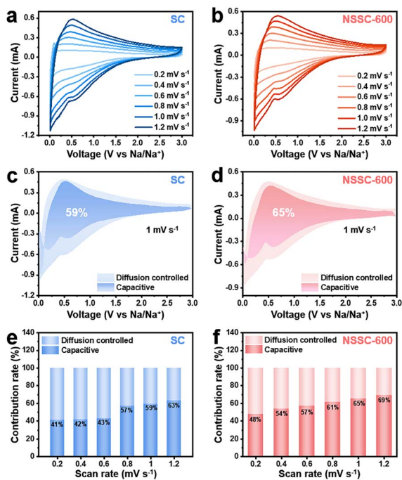
Fig. 6 CV curves of (a) SC and (b) NSSC-600 at the scan rates from 0.2 to 1.2 \text{mV s}^{-1} . Capacitive contribution area of (c) SC and (d) NSSC-600 at 1.0 \text{mV s}^{-1} . Capacitive contribution ratios of (e) SC and (f) NSSC-600 at the scan rates from 0.2 to 1.2 \text{mV s}^{-1} .
