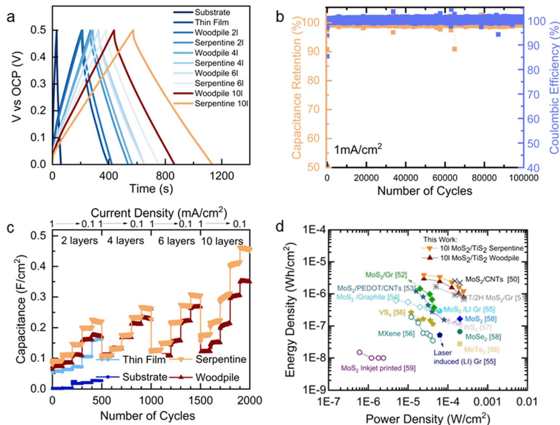
Fig. 4 Potentiometric electrochemical characterisation of printed and thin-film MoS 2 /TiS 2 microsupercapacitors. (a) Galvanostatic charge-discharge profiles at a current density of 0.1 mA cm -2 between different electrodes (substrate, thin-film, woodpile, and serpentine architectures). (b) Galvanostatic charge-discharge stability test over 100 000 cycles at a current density of 1 mA cm -2 on a 4 layered serpentine structure and (c) capacitance values extracted from galvanostatic charge-discharge at different current densities in response to the electrode geometry and added layers. (d) Ragone plot as calculated from extracted values 50-59 of CCD in TMD based devices.
