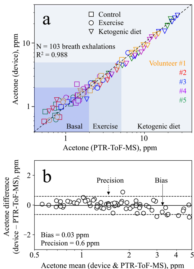
Fig. 6 (a) Scatter plot of N = 103 breath exhalations measured by the device and the PTR-ToF-MS for all five volunteers during the control (squares), the exercise (circles) and ketogenic diet (triangles) visit. Typical concentration ranges for basal acetone, after exercise, and during ketogenic diet are indicated. (b) Bland–Altman plot showing the difference in acetone concentration measured using the device and the PTR-ToF-MS as a function of the mean of both measurements for concentrations below 5 ppm. The bias and precision are indicated as solid and dashed lines, respectively.
