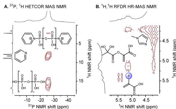
Fig. 4 (A) Characterization of the paste by ^{31}\text{P} , ^1\text{H} HETCOR MAS NMR. (B) Characterization of the paste by ^1\text{H} , ^1\text{H} RFDR HR-MAS NMR.
