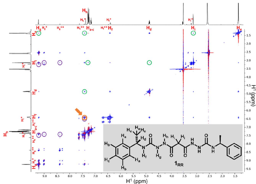
Fig. 4 600 MHz NOESY of 1_{RR} in 1,4-dioxane- d_8 . Peaks highlighted with purple circles are due to spatial interactions between protons of the major isomer and protons on the second more abundant one labelled with asterisks. Cross-peaks surrounded with green circles are due to proximity effects between hydrogen that are so far apart in that would not be observed as intramolecular interactions. The cross-peak highlighted in orange and pointed with an arrow is due to H_h being close to H_f .
