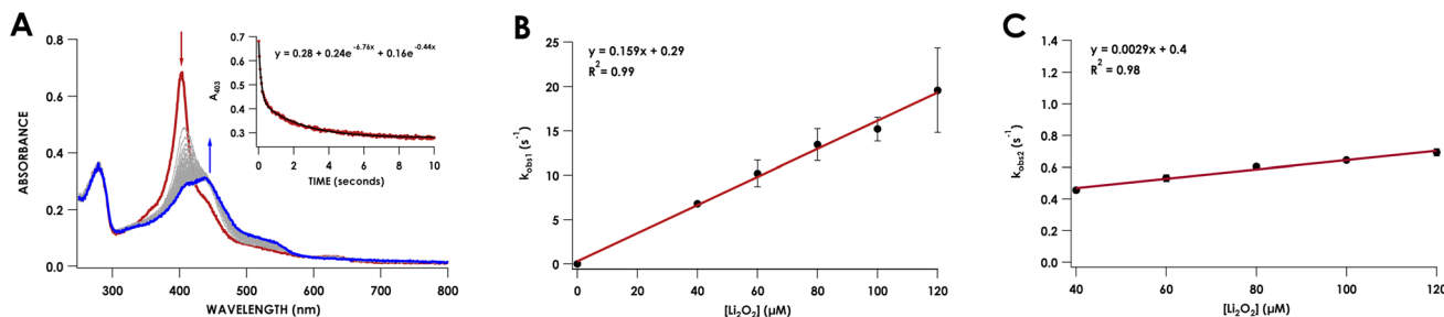
Fig. 5 (A) Stopped-flow UV/vis reaction of 10 \mu M as-isolated Phe41Ala cyt P460 and 40 \mu M Li_2O_2 in 20 mM Tris/200 mM NaCl (pH 8.0) recorded over 10 seconds. The red trace is the first scan, and the blue trace is the final scan. Scans were recorded every 4 ms and grey traces are average scans every 20 ms. The inset is the absorbance at 403 nm recorded every 4 ms fit to a double exponential. (B) Plot of k_{obs1} obtained from fitting the absorbance at 403 nm to a double exponential versus the concentration of Li_2O_2 . (C) Plot of k_{obs2} versus the concentration of Li_2O_2 .
