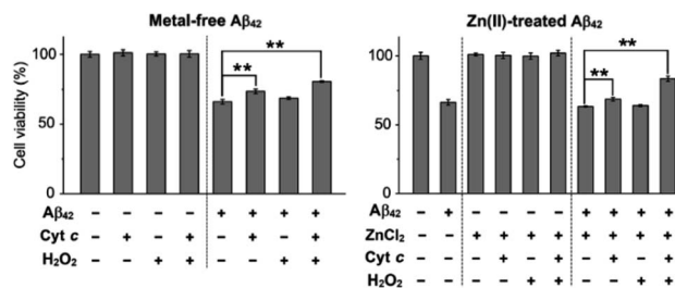
Fig. 5 Influence of Cyt c on the cytotoxicity induced by metal-free and \text{Zn(II)} -treated \text{A}\beta_{42} species with and without \text{H}_2\text{O}_2 . SH-SY5Y cells were treated with metal-free and \text{Zn(II)} -added \text{A}\beta_{42} species generated by 12 h treatment with either Cyt c , \text{H}_2\text{O}_2 , or both followed by 24 h incubation. Cell viability, determined by the MTT assay, was calculated in comparison to that with an equivalent amount of the buffered solution. Conditions: [\text{A}\beta_{42}] = 10 \mu\text{M} ; [\text{Cyt } c] = 10 \mu\text{M} ; [\text{Zn(II)}] = 10 \mu\text{M} ; [\text{H}_2\text{O}_2] = 80 \mu\text{M} ; 150 mM HEPES, pH 7.4. Data are represented as mean \pm s.e.m. **P < 0.01 by Student's t -test.
