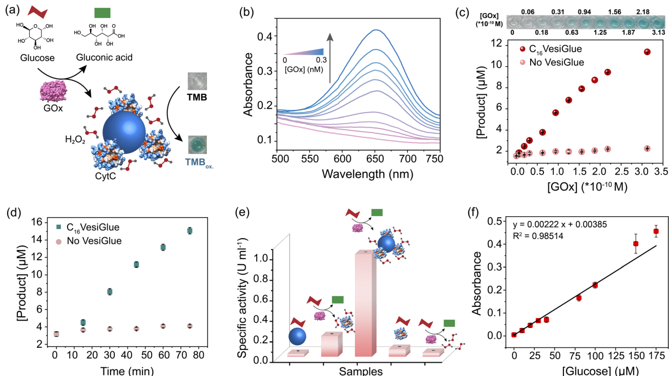
Fig. 5 Cascade reaction in the Vesiglu system. (a) Schematic of a biocatalytic cascade where glucose is oxidized by glucose oxidase (GOx), producing H 2 O 2 that serves as the substrate of CytC glued onto Vesiglu. (b) UV-vis traces of oxidized TMB (TMB ox ) with increasing GOx concentration, in the catalytic cascade. (c) C 16 Vesiglu mediated oxidation of the substrate by the biocatalytic cascade. The concentration of TMB ox is measured through the absorbance at \lambda_{\max} 650 nm. Varying concentrations of GOx (0–0.3 nM) in the presence (red) and absence (peach) of C 16 Vesiglu show the linear dependency on the enzyme concentration. The digital photos above the graph show the color of the TMB ox in presence of C 16 Vesiglu. (d) Rate of product formation (TMB ox ) in the presence (green) and absence (peach) of Vesiglu demonstrating the effect of CytC anchoring on the cascade reaction. (e) Specific activity of CytC under different conditions verifying the role of a complete system in catalyzing the cascade reactions. The shapes of (a) are used that have the same meaning. (f) The GOx/CytC/C 16 Vesiglu cascade reaction with increasing glucose concentration (0–175 μM). The black solid line represents a linear fit of the data. n = 3 technical replicates, mean \pm SD for all the studies.
