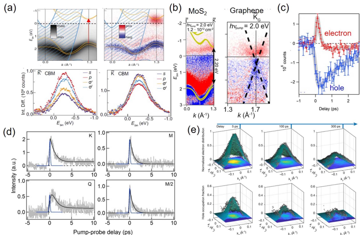
Fig. 5 Dynamics of bilayers revealed by TR-ARPES. (a) Top: ARPES of homobilayer MoS 2 and the intensity changes upon photoexcitation. Bottom: intensity difference of the CB minimum electrons at K and -K valleys, pumped with different polarizations. 132 (b) Intensity difference APPEs spectra along the \Gamma -K direction of the MoS 2 and graphene bands in a MoS 2 /graphene heterostructure, showing renormalized gap at MoS 2 . Red: increase; blue: decrease. 75 (c) Pump-probe signal of the II-band of graphene above (red) and below (blue) the equilibrium chemical potential, representing electrons and holes in the graphene layer of a WS 2 /graphene heterostructure. 133 (d) CB electron dynamics of a WS 2 /MoS 2 heterobilayer at K, Q, M/2, and M points as a function of pump probe delay. 109 (e) Distributions of electrons and holes of interlayer excitons in a WSe 2 /MoS 2 heterostructure around the K valley at different delay times. 87 The momentum space distributions of the excitons are reflective of their confinement in the real space moiré superlattice. Copyright (2019) (2020) American Physical Society. Copyright (2016) American Chemical Society. Copyright (2022) Springer Nature.
