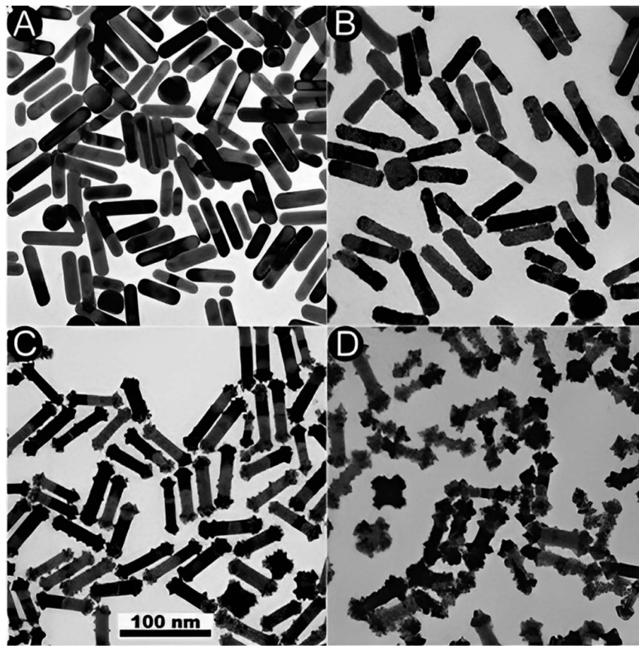
Fig. 9 (A) and (B) TEM images of the initial (GNR) and Au@Pt formed in the absence or the existence (C and D) of \text{Ag}^+ , respectively. The Pt : (G) molar ratios are 20% (C) and 100% (B, D). Reproduced with permission from ref. 124 © The Royal Society of Chemistry 2006.
