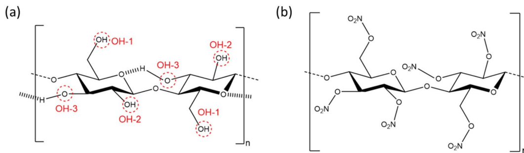
Fig. 1 Repeating dimer units of (a) cellulose and (b) NC. The dimer illustrates the intra-chain interactions in cellulose, while the glucose monomer is the more accurate chemical repeating unit. OH-1 and OH-2 represent the two most accessible hydroxyl groups on cellulose for substitution, while OH-3 is the least accessible.
