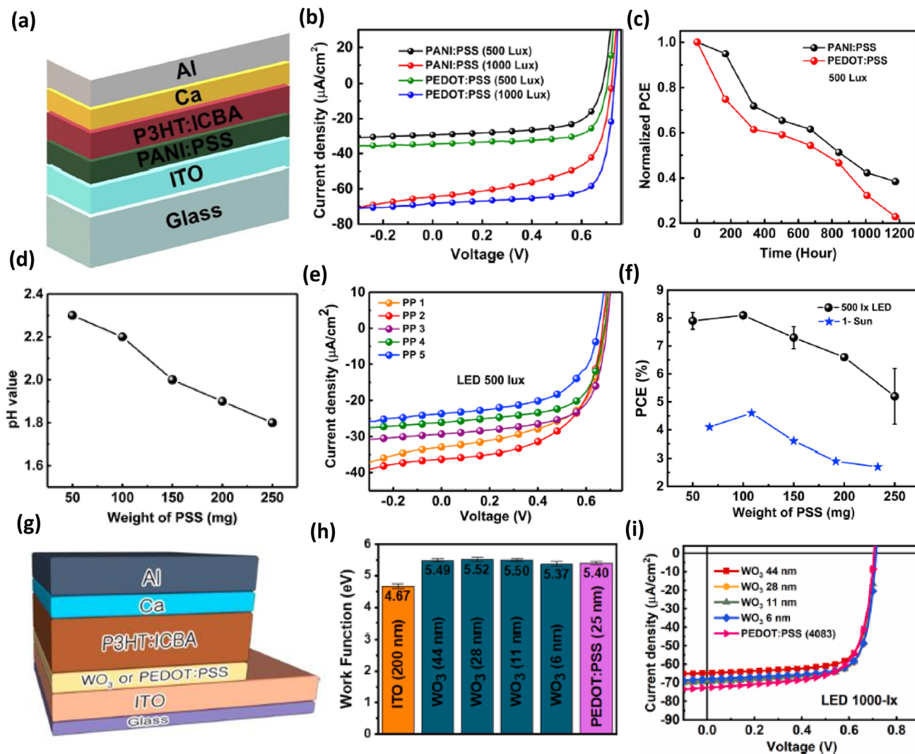
Fig. 9 (a) Architecture of an indoor OPV based on PANI:PSS HTL and P3HT:ICBA active layer, (b) J–V characteristics of the OPV operating under 500 lx and 1000 lx LED, (c) variation of normalized PCE of OPVs (PEDOT:PSS and PANI:PSS HTL-based) with their lifespan; [reproduced with permission. 44 Copyright 2020, Elsevier]. (d) Variation of pH value of PANI:PSS as per its concentration of PSS, (e) representative J–V characteristics of an OPV operating under the illumination of 500 lx LED, (f) variation of PCE value of OPVs (operating under 500 lx LED and 1 sun condition) with the doping concentration of its HTL; [reproduced with permission. 46 Copyright 2020, Elsevier]. (g) Architecture of an indoor OPV with \text{WO}_3 HTL and P3HT:ICBA active layer, (h) comparison of work function value of ITO, \text{WO}_3 and PEDOT:PSS, (i) representative J–V characteristics of OPVs (having different HTLs) operating under the illumination of 1000 lx LED; [reproduced with permission. 48 Copyright 2020, Elsevier].
