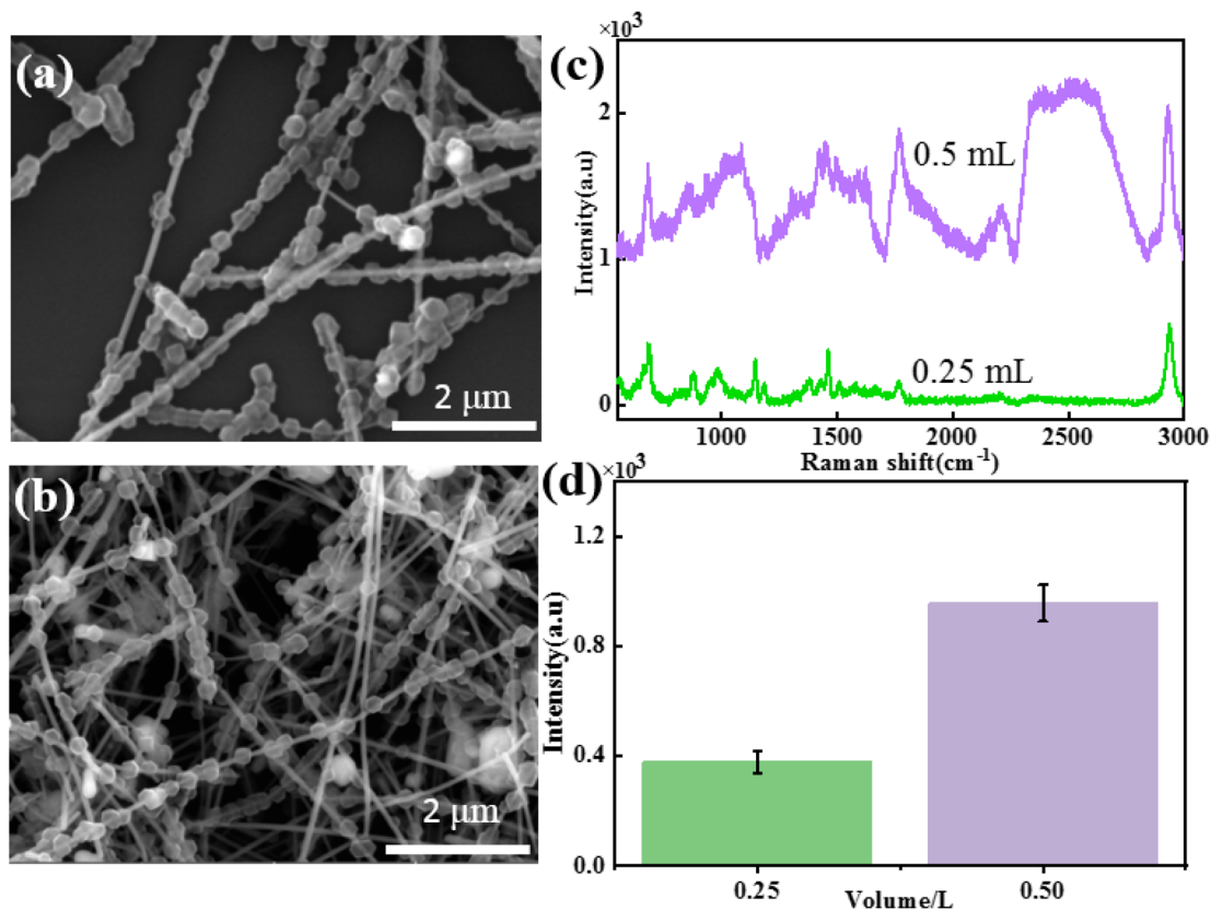
Fig. 2 SEM images of the Ag NWs@ZIF core-shell nanochains prepared with volumes of (a) 0.25 mL and (b) 0.5 mL of Ag NWs. (c) SERS spectra of methanethiol gas molecules (10 -4 M) collected on Ag NWs@ZIF substrates with different volumes of Ag NWs. (d) The corresponding histogram of the SERS intensity at 2931 cm -1 .
