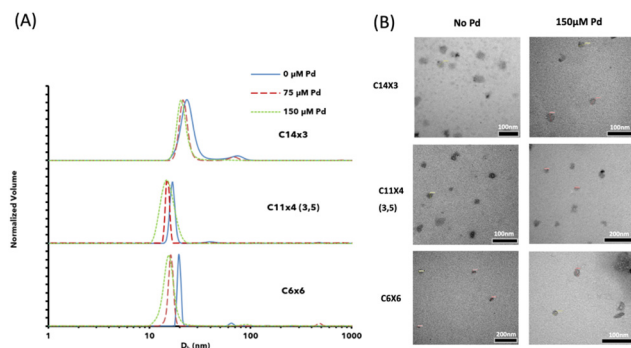
Fig. 2 (A) DLS measurements of micelles with different dendritic architectures ([amphiphile] = 320 μM) without encapsulated Pd(OAc) 2 (blue solid lines), micelles with encapsulated Pd II ([Pd(OAc) 2 ] = 75 μM) (red large-dashed lines) and micelles with encapsulated Pd II ([Pd(OAc) 2 ] = 150 μM) (green dashed lines) in PBS (pH = 7.4) at 37 °C. (B) TEM images of the micelles based on the C14x3, C11x4 (3,5) and C6x6 amphiphiles, with (right column) and without (left column) Pd(OAc) 2 salt.
