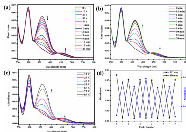
Fig. 5 UV-vis spectra of H 1 in \text{H}_2\text{O}/\text{DMSO} ( v/v = 19:1 ) solution upon exposure to different stimuli: (a) duration of UV irradiation was set to 0–20 min at 365 nm; (b) duration of vis irradiation was set to 0–20 min; (c) different temperatures of H 1 in \text{H}_2\text{O}/\text{DMSO} ( v/v = 19:1 ) solution after 20 min of UV exposure. (d) Absorbance at wavelengths of 362 nm and 450 nm under alternate UV (365 nm) irradiation for 20 min and vis irradiation for 20 min.
