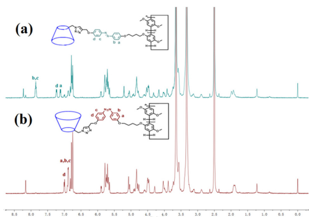
Fig. 4 ^1\text{H} NMR spectra (500 MHz, \text{DMSO}-d_6 , 25 °C) of (a) H 1 ( 2.72 \times 10^{-3} mol \text{L}^{-1} ) and (b) H 1 ( 2.72 \times 10^{-3} mol \text{L}^{-1} ) after irradiation with 365 nm UV light for 20 min.
