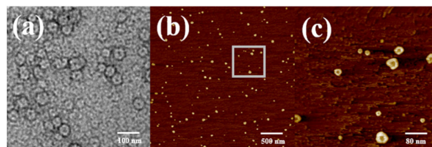
Fig. 6 (a) Negative-staining TEM images and (b) AFM images of cis - H 1 ( H 1 after irradiation with 365 nm UV light for 20 min) obtained from 3.03 \times 10^{-6} mol \text{L}^{-1} \text{H}_2\text{O}/\text{DMSO} ( v/v = 19:1 ) solutions. (c) Enlarged image of part b.
