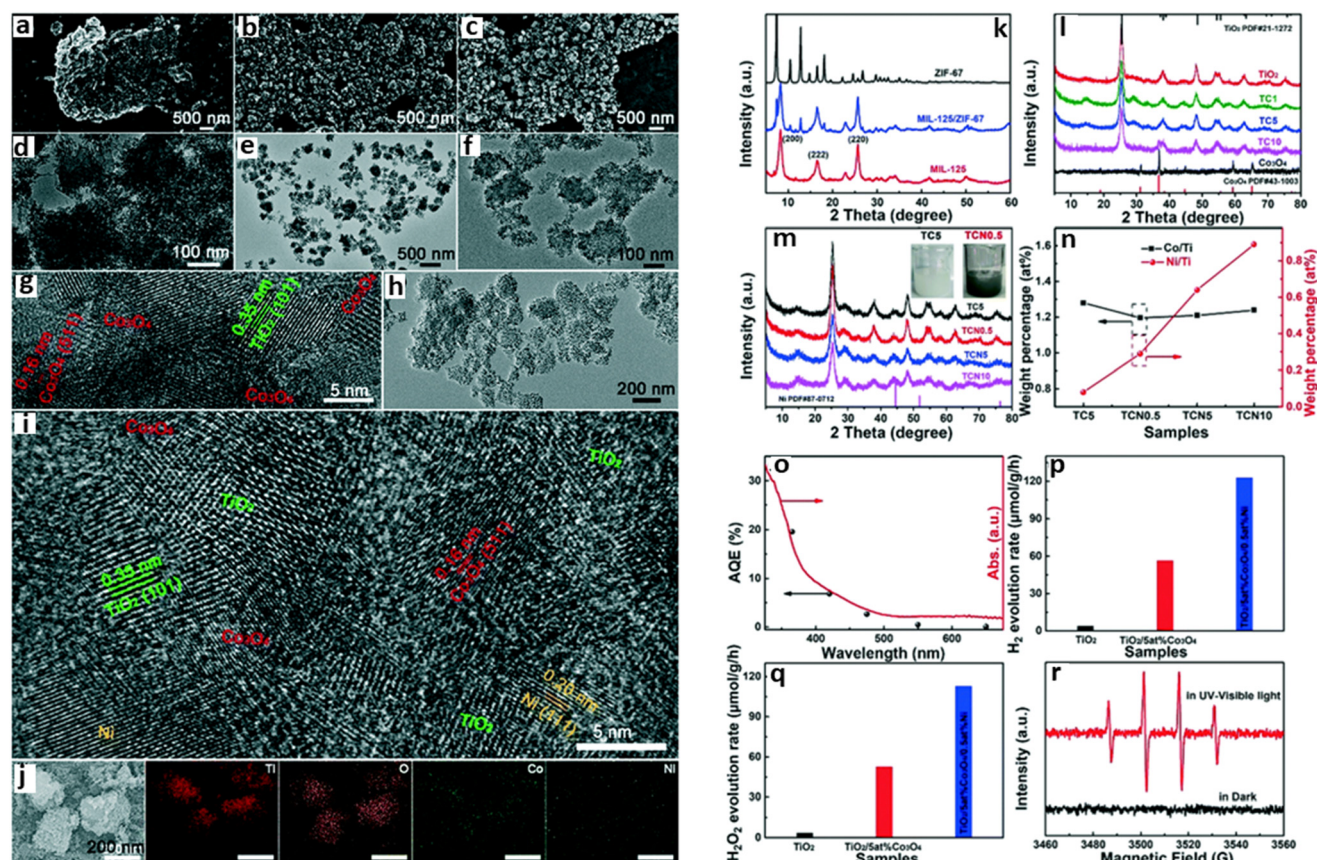
Fig. 6 SEM and TEM images of (a and d) TiO 2 , (b and e) MIL-125/ZIF-67, and (c and f) TiO 2 /5at%Co 3 O 4 , and (g) HRTEM image of TiO 2 /5at%Co 3 O 4 . The (h) TEM, (i) HRTEM, and (j) elemental mapping images of TiO 2 /5at%Co 3 O 4 /0.5at%Ni. PXRD patterns of (k) MIL-125, ZIF-67 and MIL-125/ZIF-67, (l) TiO 2 , Co 3 O 4 and TiO 2 /Co 3 O 4 heterojunctions and (m) TC5, TCN0.5, TCN5 and TCN10 composite photocatalysts and the color contrast of TC5 and TCN0.5 (inset). (n) ICP-OES experimental data of TC5, TCN0.5, TCN5 and TCN10 samples. (o) Apparent quantum efficiency (AQE) for TiO 2 /5at%Co 3 O 4 /0.5at%Ni at different monochromatic light irradiation wavelengths. The photocatalytic activities of TiO 2 , TiO 2 /5at%Co 3 O 4 , TiO 2 /5at%Co 3 O 4 /0.5at%Ni samples for (p) H 2 and (q) H 2 O 2 production without a sacrificial agent under UV-visible light. (r) EPR responses of the DMPO-OH spin adduct in TiO 2 /5at%Co 3 O 4 /0.5at%Ni. 71
