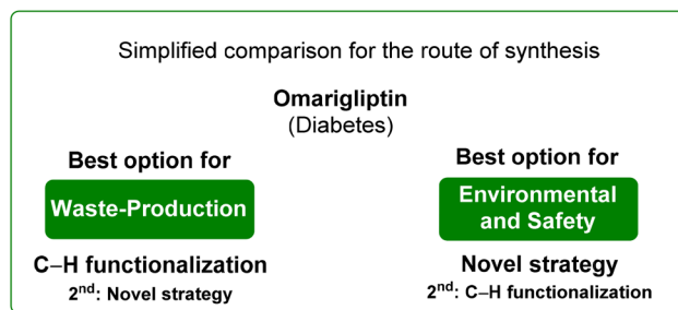
Scheme 17 Summarised assessment for omarigliptin synthesis.
