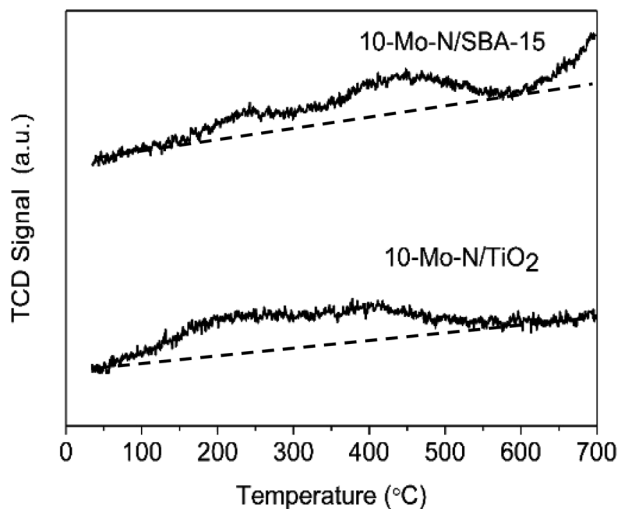
Fig. 7 H 2 -TPD profiles of 10-Mo-N/SBA15 and 10-Mo-N/TiO 2 .
