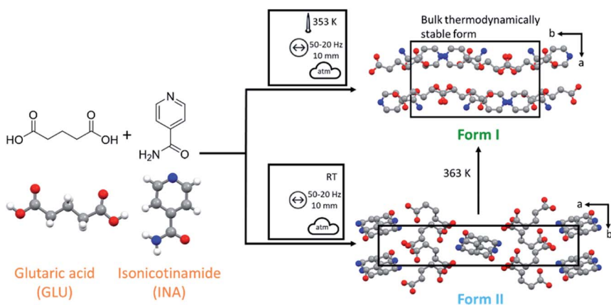
Fig. 1 Reaction scheme for the cocrystal mechanosynthesis of GLU and INA. Form I (ref. 27) and Form II viewed along the crystallographic c-axis. Mechanochemical nomenclature is taken from ref. 39. Atoms are coloured as follows: carbon (grey), oxygen (red) and nitrogen (blue).
