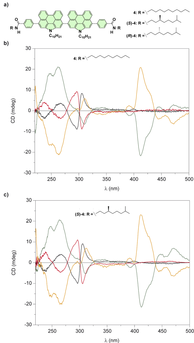
Fig. 4 (a) Chemical structures of bis( N -annulated) perylene-3,4,9,10-tetracarboxylic diimides 4 . CD spectra of all stereoisomers of 4 (b) and ( S )- 4 (c) in a molecularly dissolved state (black and red lines; CH 2 Cl 2 , c T = 10 μM, 298 K) and in the aggregated state (green and orange lines); 95/5 cyclohexane/CH 2 Cl 2 , c T = 10 μM, 298 K (reproduced from ref. 52 with permission from the American Chemical Society, copyright 2015).
