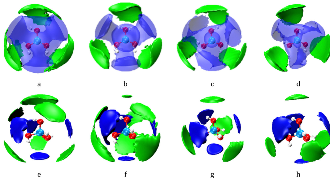
Fig. 6 SDF surfaces showing the probability density for correlations of hydration water molecules with respect to the central [B(OH)_3] and [B(OH)_4^-] moieties. The blue and semitransparent lobes represent water molecules in the first (direct) hydration shell, whilst the green lobes represent water molecules in the second (indirect) hydration shell. For the first and second hydration shells, the isosurfaces have been selected to show the distribution of neighbours with the threshold selected to show the most probable 30% and 20% of neighbour locations respectively. (a and b) The cis - B(OH)_3 in aqueous K_2B_4O_7 solutions with WSR = 100 and 60; (c and d) the trans - B(OH)_3 in aqueous K_2B_4O_7 solutions with WSR = 100 and 60; (e and f) the B(OH)_4^- anion in aqueous K_2B_4O_7 solutions with WSR = 100 and 60; (g and h) the B(OH)_4^- anion in aqueous KBO_2 solutions with WSR = 60 and 20; the pink, red, and white balls in the center respectively represent B, O, and H atoms of B(OH)_3 or B(OH)_4^- . The first (direct) hydration shell of B(OH)_3^- is in the range 2.6 to 4.5 Å, and the second shell is in the range 4.6 to 5.2 Å. The first (direct) hydration shell of B(OH)_4^- is in the range 2.6 to 3.9 Å, and the second shell is in the range 3.7 to 4.8 Å.
