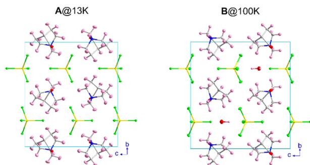
Fig. 1 (Left) View of the unit cell of compounds A (at 13 K), and B (at 100 K). (Right) The displacement ellipsoids are shown with 50% probability. Colour codes: yellow, iron; green, chloride; grey, carbon; blue, nitrogen; red, oxygen; and pink, hydrogen.
