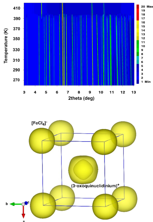
Fig. 2 (Top) Temperature evolution of the synchrotron powder diffraction data of compound A from 260 to 420 K. (Bottom) Calculated Fourier maps in the plastic phase derived from the refinement of the experimental data at 420 K (phase A I , plastic phase) using a spherical shell refinement.
