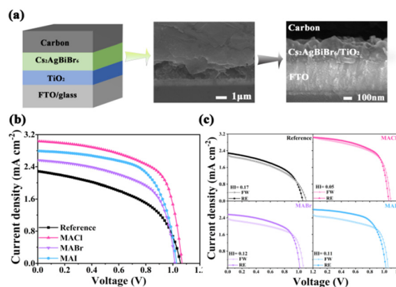
Fig. 2 (a) Scheme and SEM sectional images of the device structure. (b) J - V curves of the champion devices. (c) RE and FW J - V curves for the best devices.
