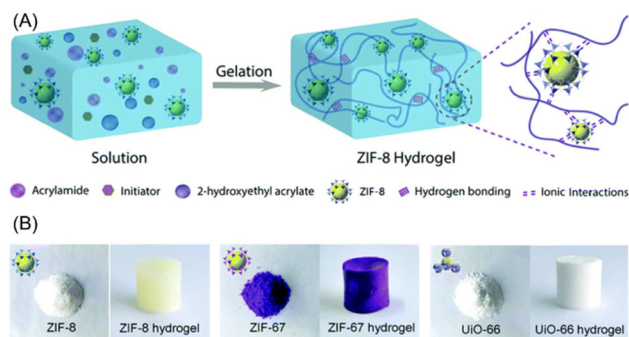
Fig. 2 (A) Synthetic strategy of adding the MOFs to a pre-polymer solution with the required monomers and initiators. Gelation gave the MOF-hydrogel hybrid. (B) The MOF powders and composite MOF-hydrogels as synthesized. Reproduced from ref. 32 with permission from the Royal Society of Chemistry, copyright 2019.
