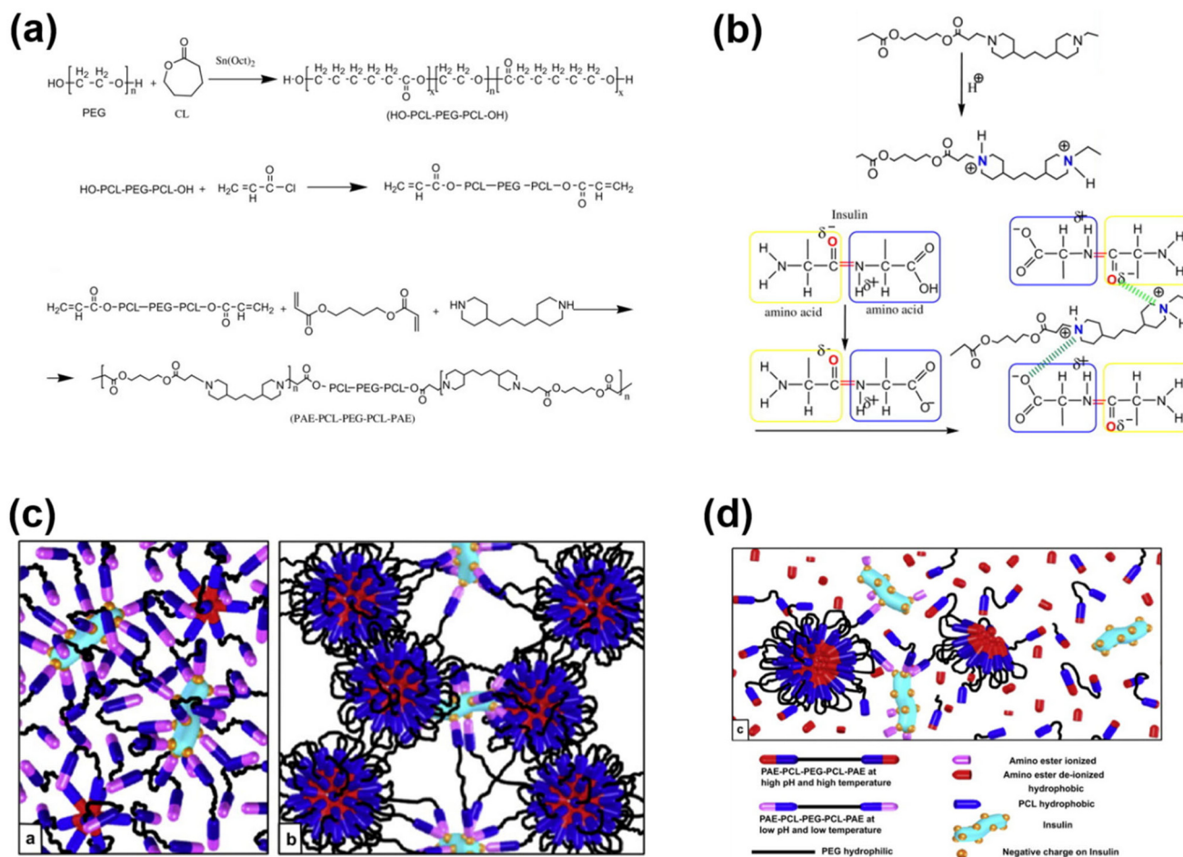
Fig. 4 (a) Synthesis route to prepare pH-responsive cationic pentablock copolymers. (b) Ionization of a cationic polymer at low pH and its interaction with anionic residues of insulin. (c) and (d) Schematic illustration of an insulin-loaded pH-responsive hydrogel and its sustained release characteristics. 65 Reproduced from ref. 65 with permission from Elsevier Limited, Copyright 2008.
