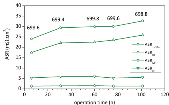
Fig. 7 Long-term operation test of LSC75–GDC MW 25 cathode at 700 °C during 101 h under synthetic air flow. The evolution of each component with time shows the origin of the increment in ASR TOTAL observed during the first hours of operation. The inserted numbers indicate the temperature of the sample in °C when the measurement was performed.
