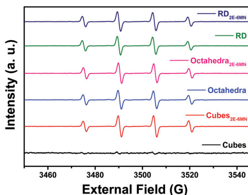
Fig. 6 EPR spectra of photoirradiated pristine and 2E-6MN-functionalized Cu 2 O polyhedra.
