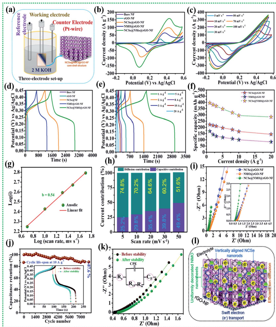
Fig. 5 (a) Schematic representation of the three-electrode system, (b) CV performance of various electrodes at a scan rate of 10 mV s -1 , (c) CV performance of the NCSe@NMO@rGO-NF at different scan rates, (d) GCD performance of various electrodes at a current density of 1 A g -1 , (e) GCD performance of NCSe@NMO@rGO-NF at different current densities, (f) rate capability curves, (g) relationship between log( i ) vs. log( v ) of the NCSe@NMO@rGO-NF electrode, (h) diffusion and capacitive current contributions of the NCSe@NMO@rGO-NF electrode, (i) EIS curves of the as-fabricated various electrodes, (j) cycling performance of the NCSe@NMO@rGO-NF electrode at a current density of 1 A g -1 , (k) EIS in the form of a Nyquist plot of the NCSe@NMO@rGO-NF electrode before and after cycling, and (l) schematic representation of the electrochemical mechanism of the NCSe@NMO@rGO-NF electrode.
