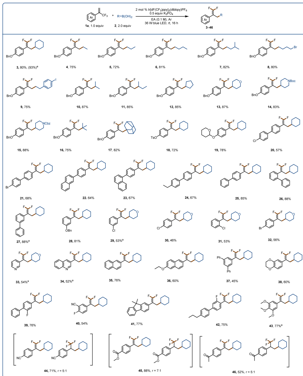
Fig. 3 Substrate scope of the defluorinative alkylation reaction. Reaction conditions, unless otherwise noted: 1 (0.2 mmol), 2 (0.4 mmol), K_3PO_4 (0.1 mmol, 0.5 equiv.), \text{Ir}[\text{d}(\text{CF}_3)\text{ppy}]_2(\text{dtbbpy})\text{PF}_6 (2 mol%), ethyl acetate (EA, 2.0 mL), Ar, 36 W blue LED, rt, 16 h. a K_3PO_4 (0.2 mmol, 1.0 equiv.).
