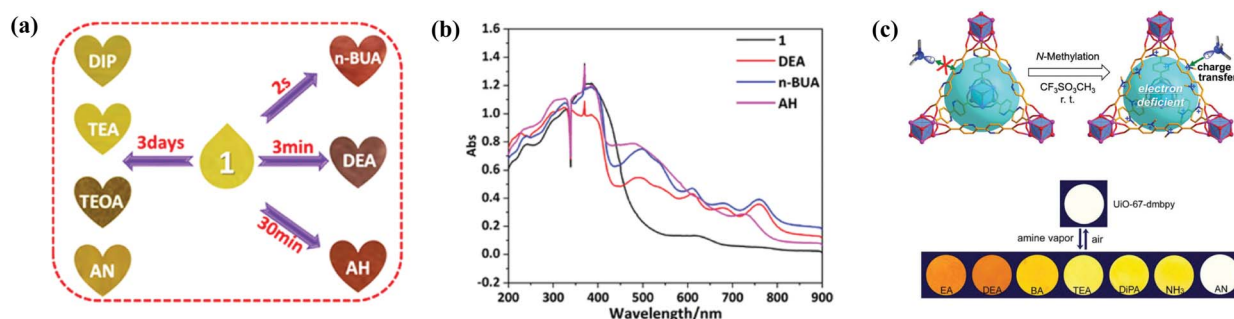
Fig. 4 (a) Color change and response time of [\text{Zn}(3\text{-DPMNI})_{0.5}(\text{NDC})] (denoted as 1 in the figure and following text), ( \text{H}_2\text{NDC} = 2,6-naphthalenedicarboxylic acid and 3-DPMNI = N,N' -bis(3-pyridylmethyl)-1,4,5,8-naphthalene diimide) in the presence of different organic amines. Figures adapted from ref. 105. (c) Structure of N -methylated UiO-67-dmbpy and its reversible colour change when deposited UiO-67-dmbpy was exposed to amine vapours. n -BUA(in a)/BA(in c) = butylamine, DEA = diethylamine, AH = hydrazine, DIP(in a)/DiPA(in c) = diisopropylamine, TEA = triethylamine, TEOA = triethanolamine, AN = aniline, and EA = ethylamine. Figures adapted from ref. 100.
