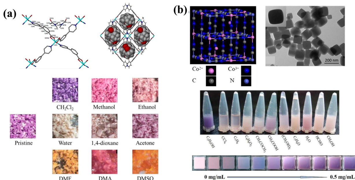
Fig. 3 (a) Coordination environment of Co(II), packing of [\text{Co}_3(3,4\text{pba})_2 \cdot (\text{H}_2\text{O})] \cdot 1/2\text{DMF} \cdot \text{H}_2\text{O}_n ; and pictures of powdered samples after exposure to different solvents. Figures adapted from ref. 126. (b) Structure of \text{Co}_3[\text{Co}(\text{CN})_6]_2 and TEM image of the nanoparticles; the colour of \text{Co}_3[\text{Co}(\text{CN})_6]_2 films changes from pink to purple gradually with an increasing ethanol concentration gradient. Adapted with permission from ref. 96.
