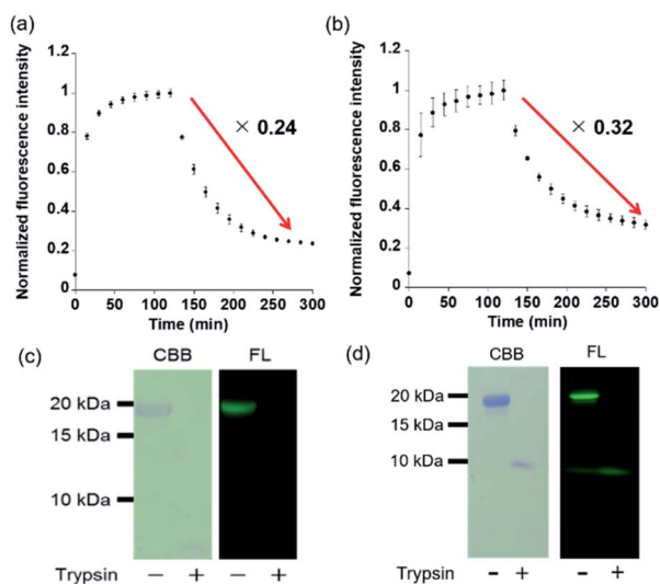
Fig. 5 (a & b) Protein degradation detected from the “OFF–ON–OFF” fluorescence response of F5-DNB2. (a) PYP 3R (6.0 \mu M) and (b) PYP NQN (6.0 \mu M) incubated with F5-DNB2 (5.0 \mu M) for 120 min and then reacted with (a) trypsin (0.3 \mu M) or (b) trypsin (0.5 \mu M) in 20 mM HEPES buffer (pH 7.4), 150 mM NaCl, and 1.0% DMSO at 37 ^{\circ} C. Fluorescence intensities recorded using excitation and emission wavelengths of: (a) PYP 3R : 500 and 523 nm; and (b) PYP NQN : 500 and 521 nm, respectively. Error bars denote SD, n = 3 . (c & d) SDS-PAGE analyses of protein degradation products. (c) PYP 3R (20 \mu M) & (d) PYP NQN (20 \mu M) labeled with F5-DNB2 (15 \mu M) for 120 min and then reacted with (c) trypsin (1.0 \mu M) or (d) trypsin (1.5 \mu M) in 20 mM HEPES buffer (pH 7.4), 150 mM NaCl and 1.0% DMSO at 37 ^{\circ} C for 180 min. CBB = Coomassie Brilliant Blue; FL = Fluorescence.
