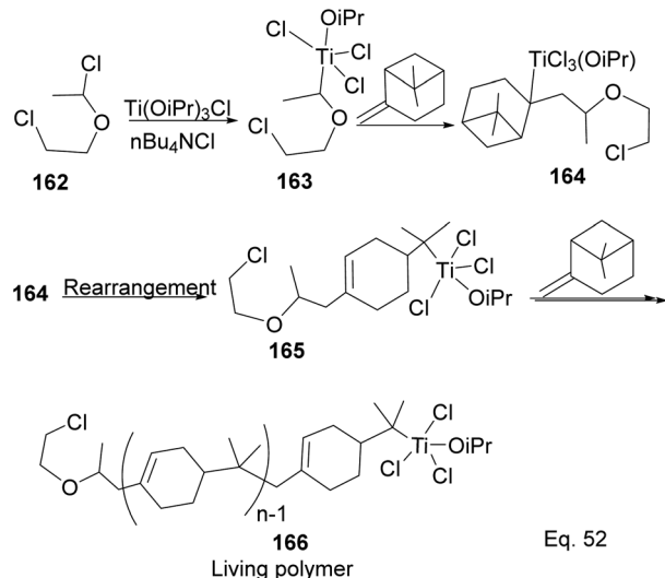
Scheme 46 Ti(iOPr)Cl 3 -promoted cationic polymerization of \beta -pinene.
