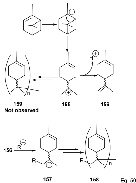
Scheme 44 Metal-based Lewis acid promoted cationic polymerization of α-pinene.
