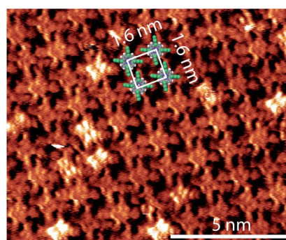
Fig. 4 2HTFPP after annealing to 200 °C. The unit cell has dimensions of 1.6 \text{ nm} \times 1.6 \text{ nm} and the monolayer has a packing density of 0.38 molecules per \text{nm}^2 . The bright double-dot features are doubly stacked porphyrins, the start of a second layer. The image was taken with a bias voltage of -10.0 mV and a tunneling current of 10 pA.
