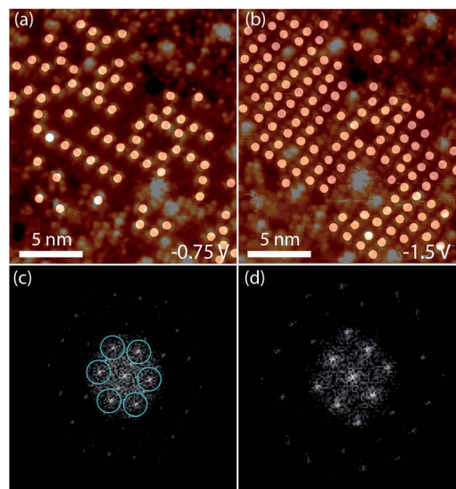
Fig. 3 (a) Circles placed over each 2HTFPP molecule with bright double dot features at -0.75 V and (b) -1.5 V (c) is FFT of (a) showing hexagonal order (d) is FFT of (b) showing rectangular order.
