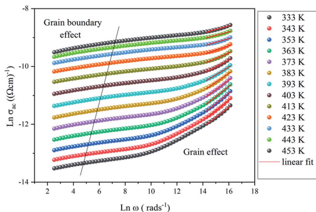
Fig. 13 The variation of \text{Ln}(\sigma_{\text{ac}}) versus \text{Ln}(\omega) at different temperatures for the \text{NaCu}_{0.2}\text{Fe}_{0.3}\text{Mn}_{0.5}\text{O}_2 compound.
