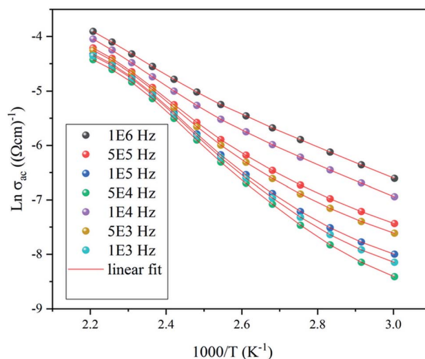
Fig. 15 The variation of \text{Ln}(\sigma_{\text{ac}}) versus 1000/T .
