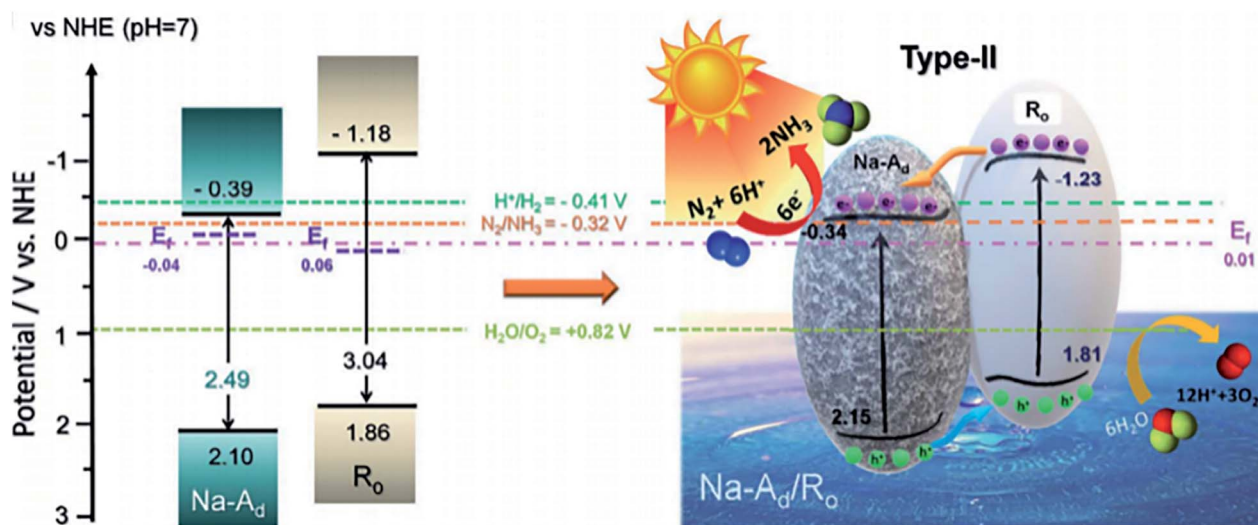
Fig. 5 Energy band structure of disordered TiO 2 (short for Na-A d ) and ordered TiO 2 (represented by R o ) as well as the reaction mechanism. This figure has been adapted from ref. 92 with permission from Royal Society of Chemistry, copyright 2020.
