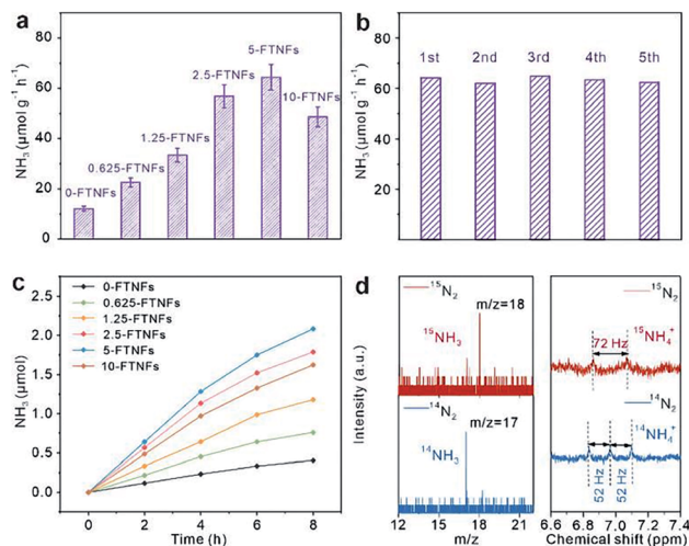
Fig. 7 (a) Performance of Fe doped \text{TiO}_2 (x-FTNFs, where x is the loading of Fe) in PNF. (b) Stability test of 5-FTNFs in PNF. (c) Time-dependent \text{NH}_3 production over x-FTNFs. (d) Isotope labeling experiment (left panel) and ^1\text{H} -NMR (right panel) of the products. This figure has been adapted from ref. 99 with permission from Royal Society of Chemistry, copyright 2021.
