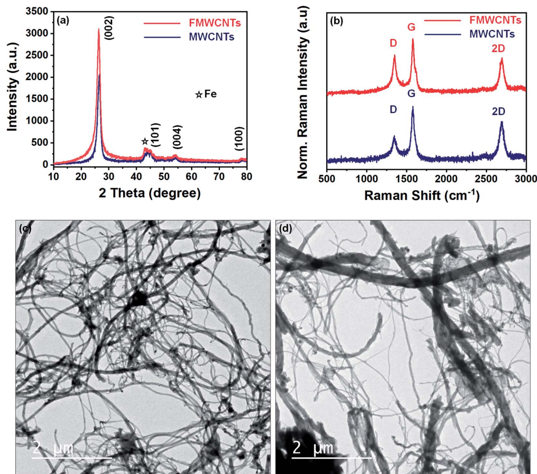
Fig. 3 (a) Typical XRD patterns of the as-synthesized and acid treated MWCNTs. (b) Raman spectra of the as-synthesized and acid treated MWCNTs. (c) and (d) TEM images of the as-synthesized and acid treated MWCNTs, respectively.
