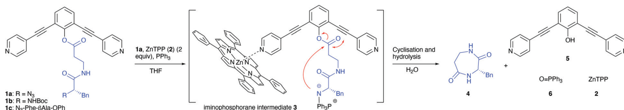
Fig. 1 The concept of site-isolation of an activated peptide by self-assembly by porphyrin-pyridyl coordination to form a cavity, possibly leading to more efficient formation of cyclic dipeptide.
